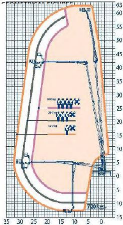
COMPLETELY OPEN CROSSBEAMS
